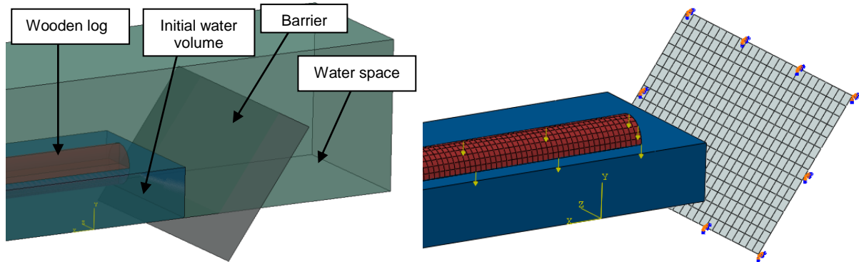
Fig. 3 CAD model of barrier (left), numerical simulation assembly (right).
