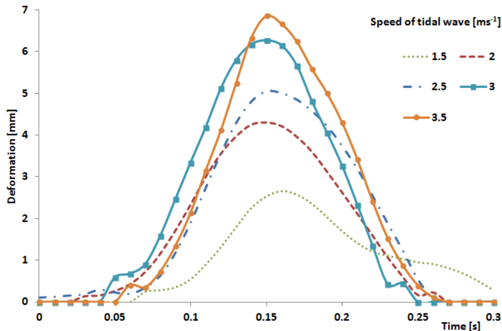
Fig. 5 Deformation of the barrier
