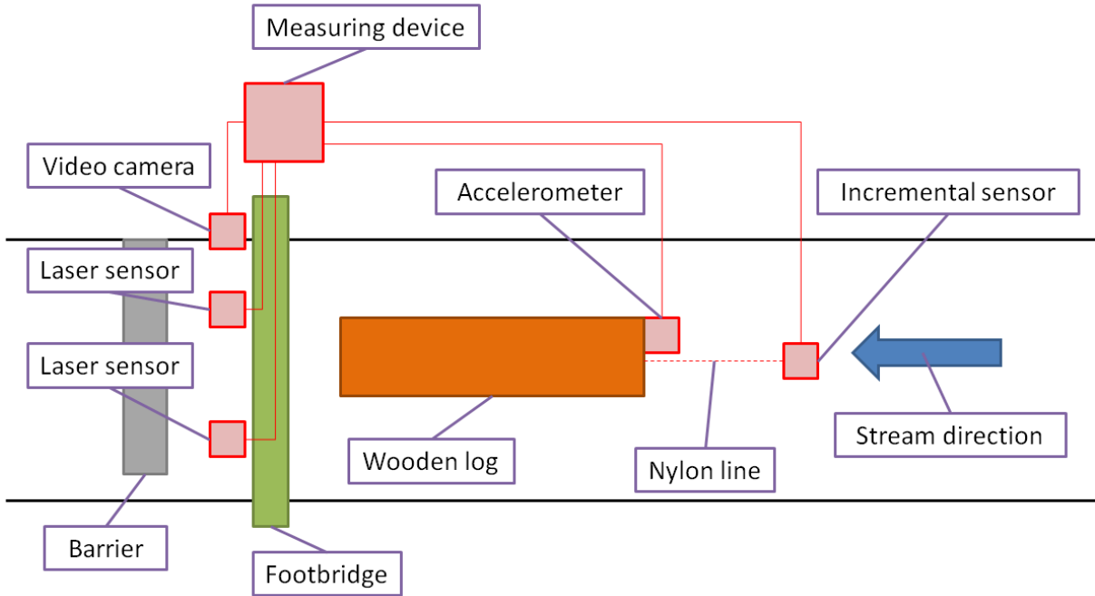
Fig. 2 The layout of experiment.
